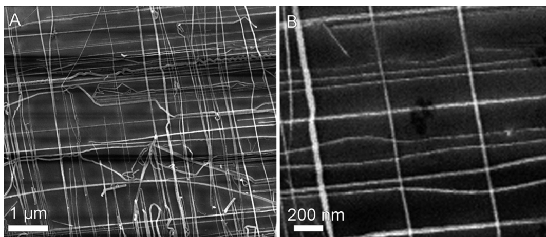
Figure 8. Nanowire crossbar arrays produced by transferring one array of guided GaN nanowires onto a similar array at 90° with one another.
