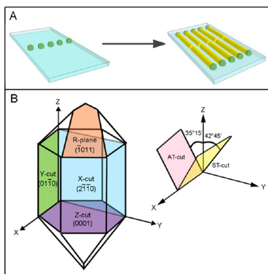
Figure 1. (A) Schematic representation of the guided growth of horizontal nanowires selectively from a catalyst pattern in specific directions. (B) Different planes of quartz on which GaN nanowires were horizontally grown in this work.
