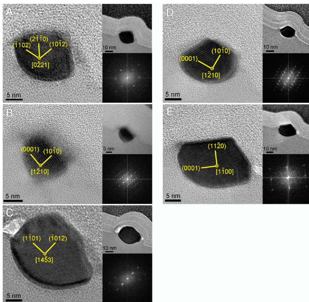
Figure 3. Cross-sectional TEM images of GaN nanowires grown on (A–C) X-cut and (D,E) Y-cut quartz. The upper-right insets show a low-magnification general view of the same cross section, and the lower-right insets show Fourier transform of the nanowires' section in the TEM image. The images exemplify the most common axial orientations of the nanowires that were observed on each substrate. See the Supporting Information for more TEM images of the less common orientations, on both X-cut and Y-cut quartz.
