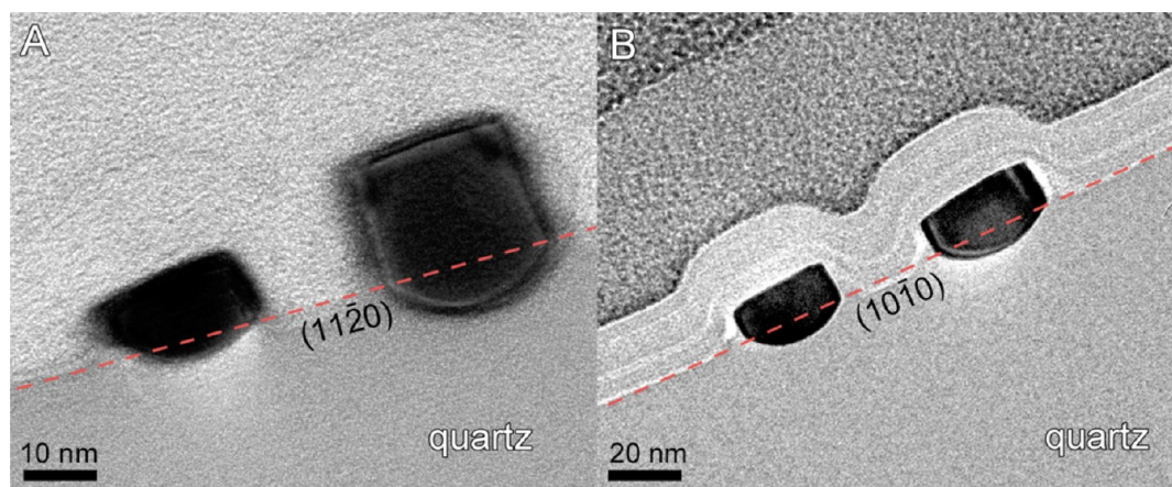
Figure 4. Cross-sectional TEM images reveal that the nanowires are slightly embedded in both the (A) X-cut and the (B) Y-cut quartz. Their shape is round at the interface with the quartz and faceted at the top. The transition between the rounded area and the faceted area occurs at the baseline of the quartz surface (indicated by the dashed red line).
